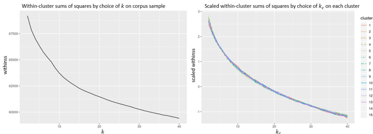
Figure 1: The curvature of the k-means objective function begins to flatten out at k = 15 for clusters and k_c = 15 for subclusters.
